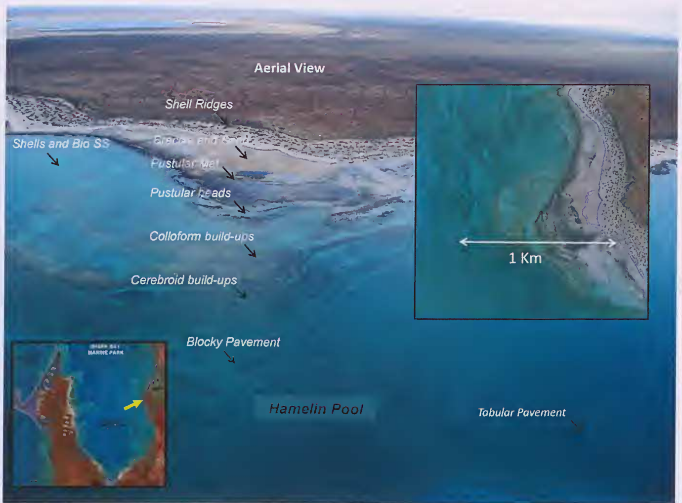
Figure 7 Hamelin Pool microbial substrates.
